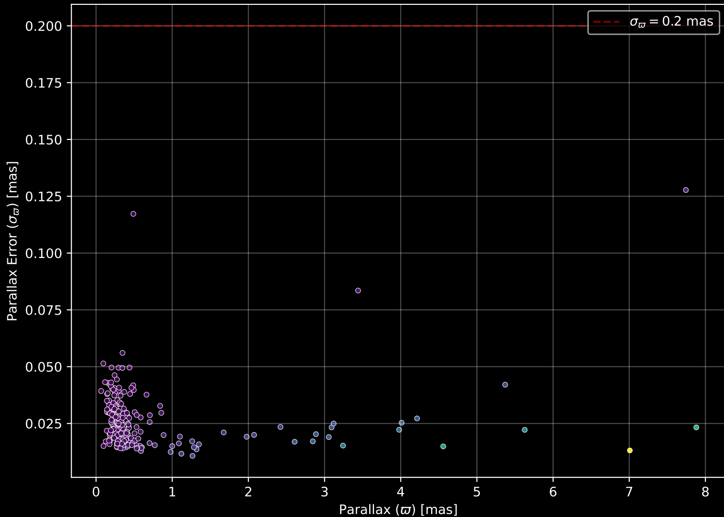
APOGEE DR17 Field: [143-04] Parallax Quality (n= 204)
