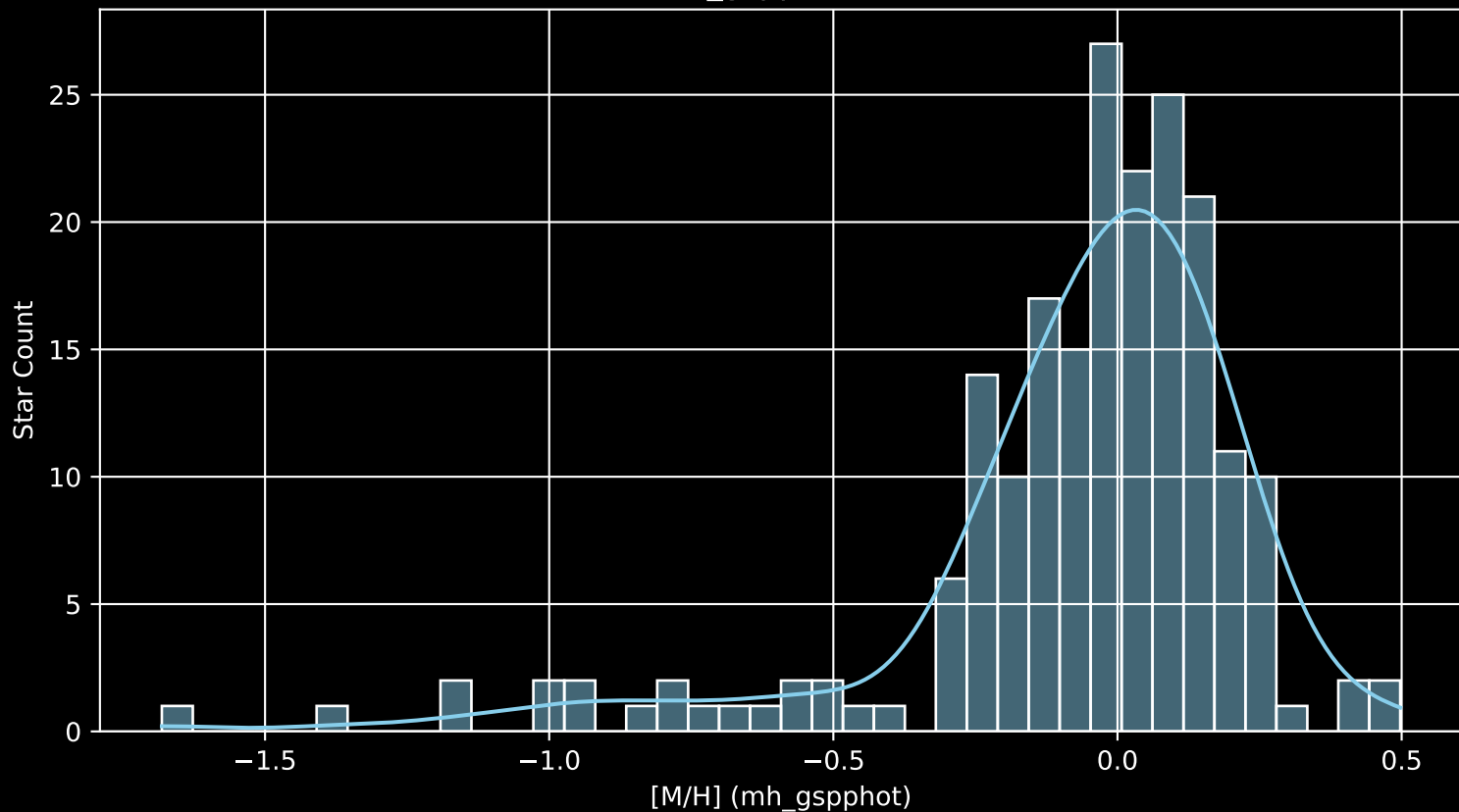
APOGEE DR17 Field: [143-04 [M/H] (mh_gspphot) (n= 203)
