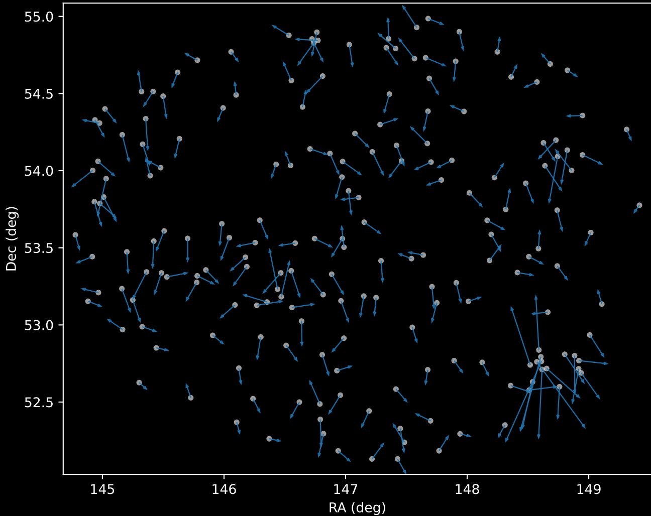
APOGEE DR17 Cluster 0 Proper Motion Vectors (n=192)
