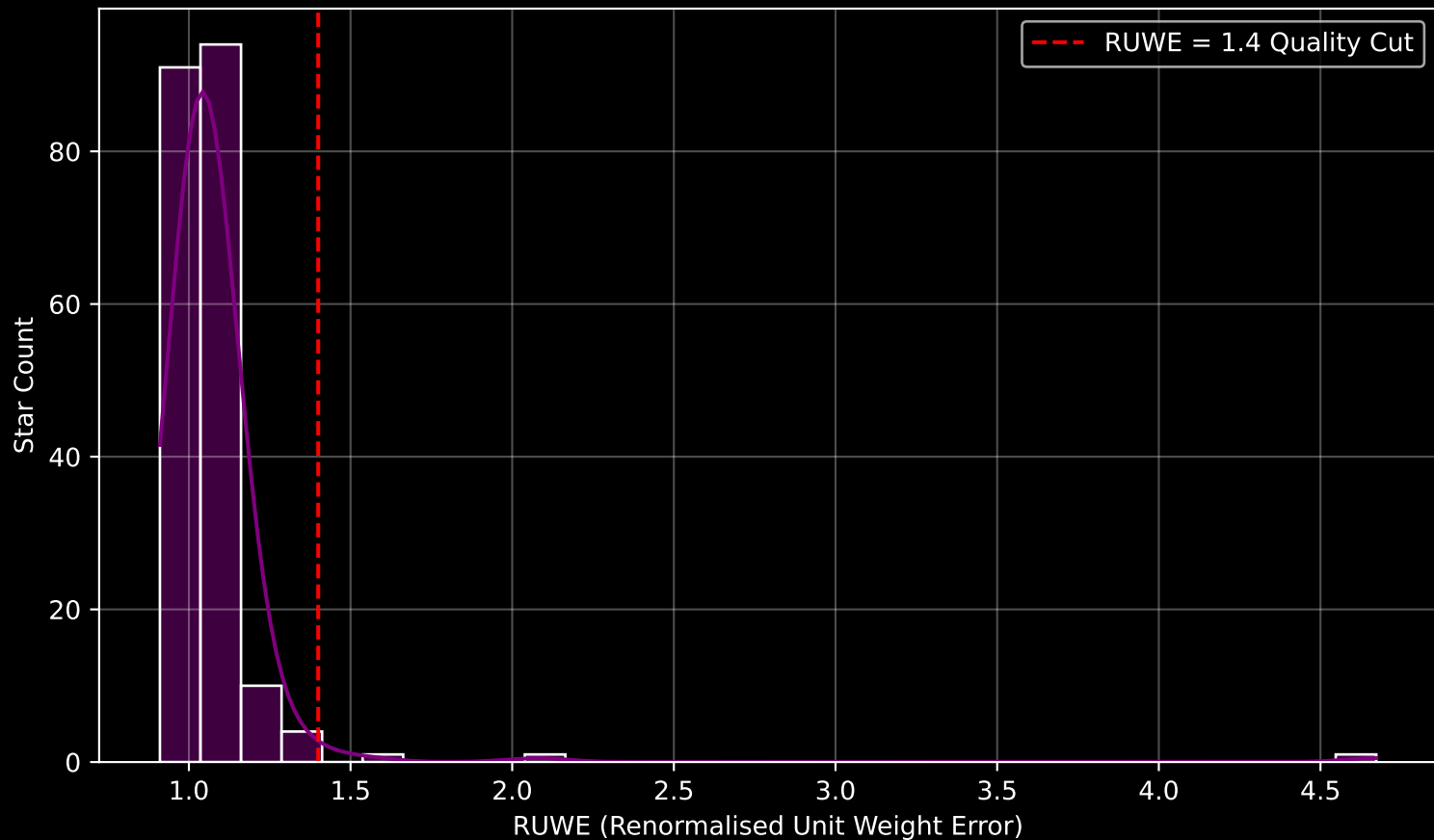
GAPOGEE DR17 Field [143-04] RUWE Distribution (n= 202)
