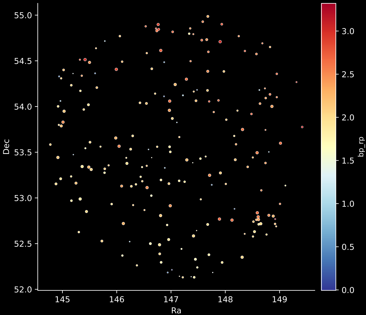
APOGEE DR17 Field: [143-04] Stars: 204
