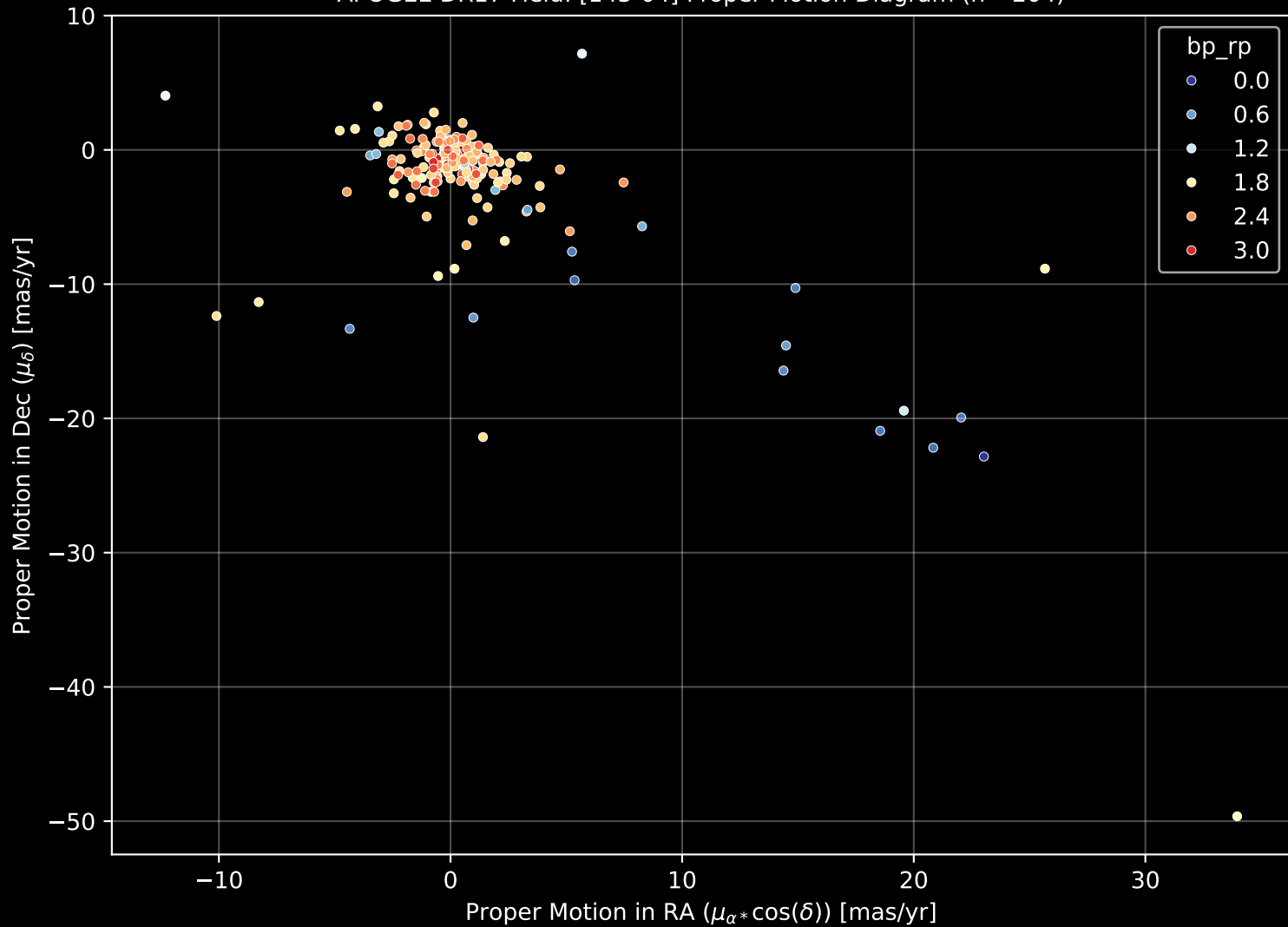
APOGEE DR17 Field: [143-04] Proper Motion Diagram (n= 204)
